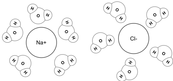
Figure 3: Hydration Spheres
