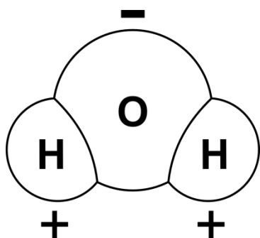
Figure 1: Water is polar molecule
