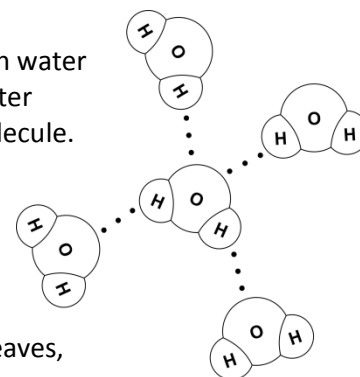
Figure 2: Hydrogen Bonding
